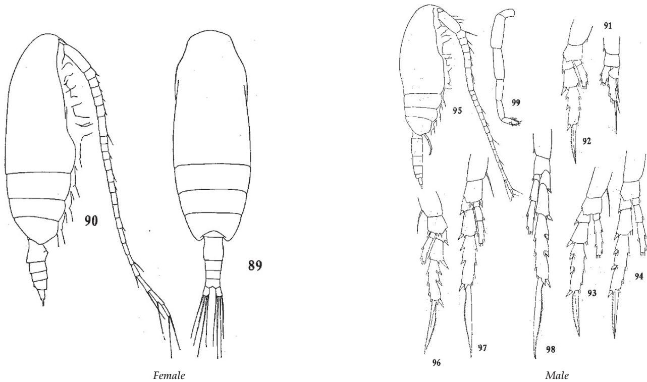
Ctenocalanus vanus Giesbrecht, 1888
