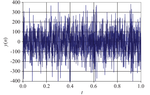
Fig. 9. Propeller modulated noise.
