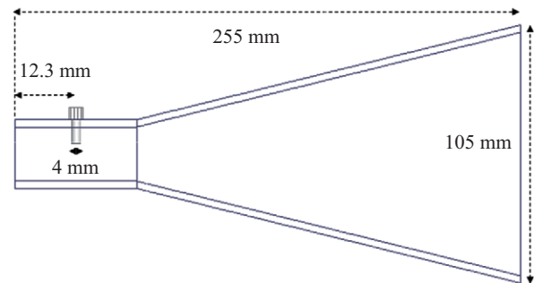
Fig. 3. Pyramidal horn antenna dimensions (side view).
