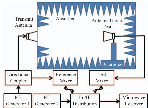
Fig. 6. Block diagram of a typical antenna measurement system.
