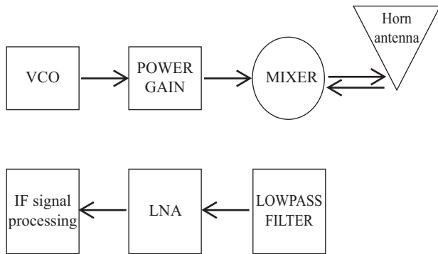
Fig. 1. Block diagram of the proposed WLRs prototype.
