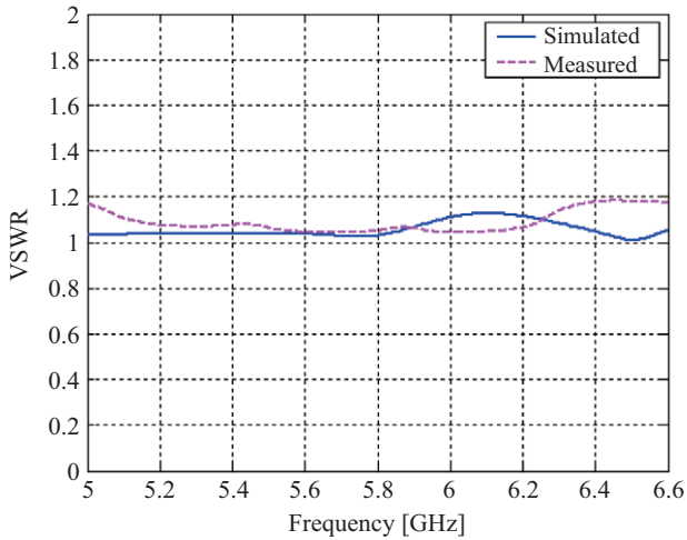
Fig. 7. Voltage standing wave ratio of the pyramidal horn antenna.
