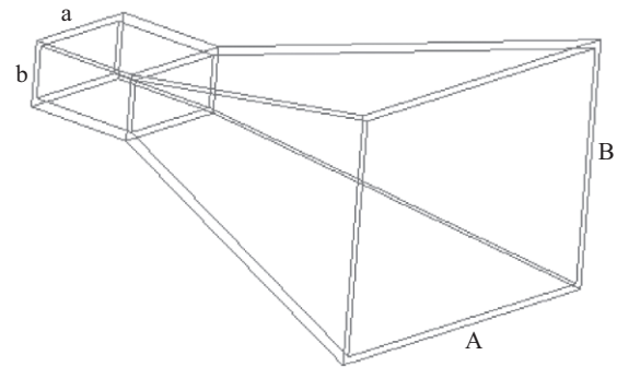
Fig. 2. Model of a pyramidal horn antenna.
