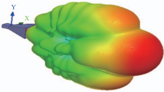
Fig. 11. 3D plot of the radiation pattern of the pyramidal horn antenna.
