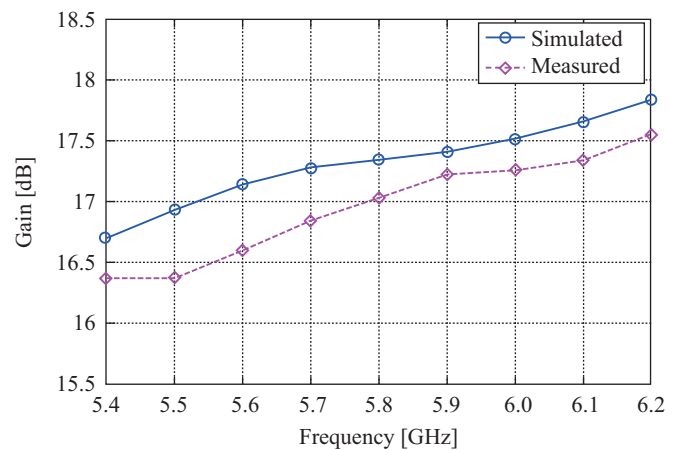
Fig. 10. Gain characteristics of the pyramidal horn antenna.
