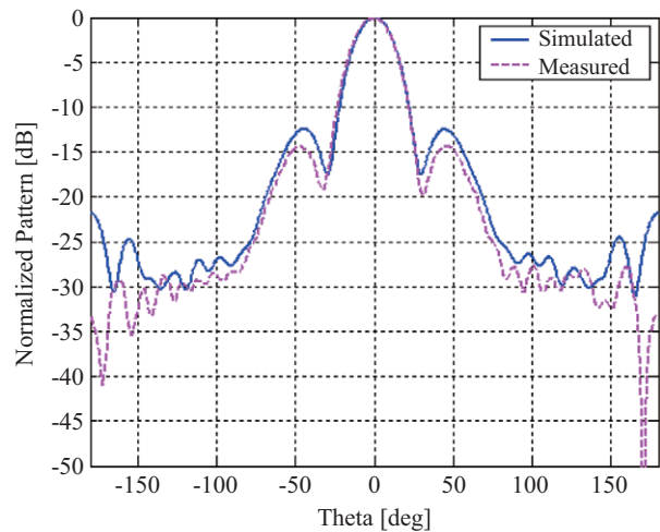
Fig. 8. E-plane radiation pattern of the pyramidal horn antenna.
