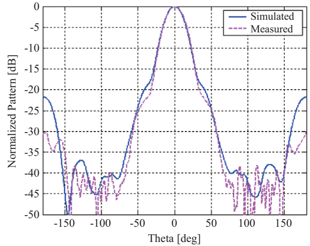
Fig. 9. H-plane radiation pattern of the pyramidal horn antenna.
