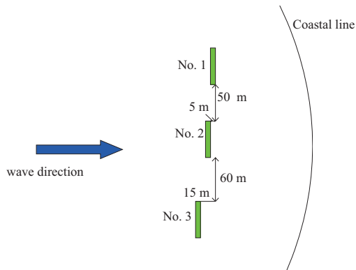
Fig. 5. Layout of three flexible devices: the second device was moved 5 m further into the sea than the first, and the third one moved 15 m.
