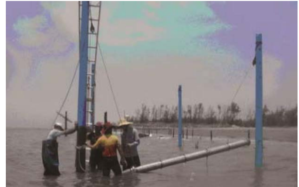
Fig. 6. Assembling the concrete posts with spring-pipes.
