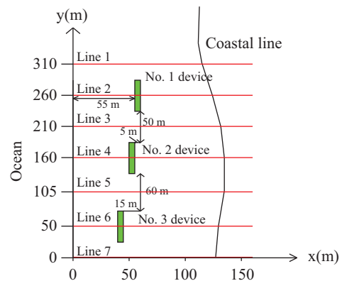
Fig. 18. Assigned profile lines for studying temporal and spatial variations in beach elevation.
