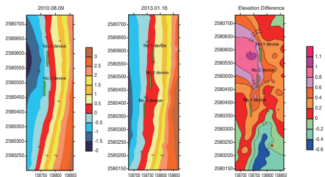
Fig. 17. Comparison of beach elevation contours measured on Aug. 9, 2010 and Jan. 16, 2013. The beach around these three breakwaters has sediment accumulation, but the south part about 50 meters away from No. 3 breakwater (out of breakwater protection) still suffers sediment erosion.
