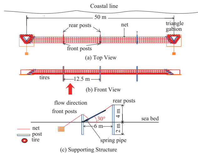
Fig. 4. Setup of the high-strength-net flexible breakwater used in the experimental field study.
