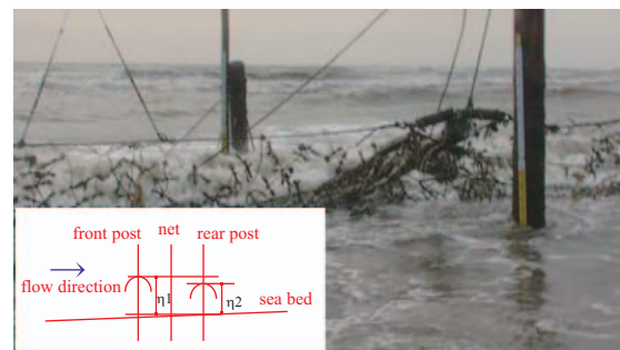
Fig. 9. Wave-level measurements taken at the front and rear of the flexible breakwater are conducted using rulers attached to the concrete posts.
