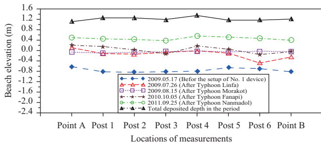
Fig. 10. Temporal variations in beach elevation measured around the No. 1 flexible breakwater, before and after device set-up.
