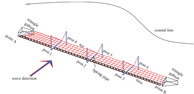
Fig. 3. Schematic diagram of a high-strength-net flexible breakwater.
