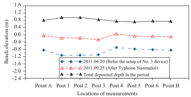
Fig. 13. Temporal and spatial variations in beach elevation around No. 3 flexible breakwater.
