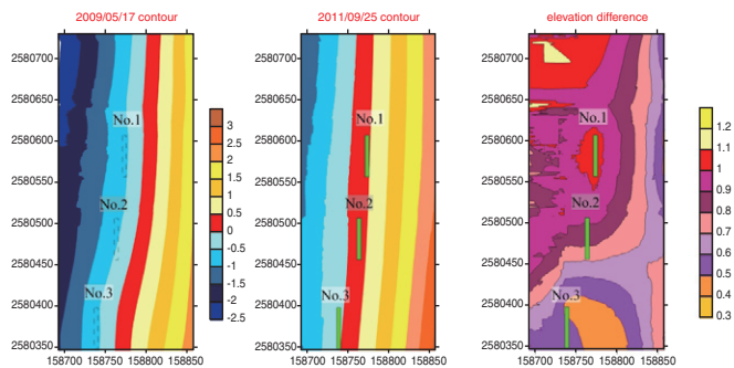
Fig. 16. Comparison of the beach contours measured on 2009/05/17 (left-hand drawing) and 2011/09/25 (central drawing), and the difference between them (right-hand drawing) after the set-up of the three devices (Unit: m).
