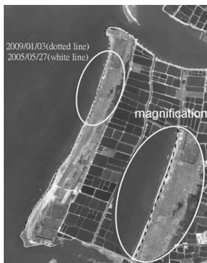
Fig. 2. Shoreline comparison based on satellite images taken on 2005/5/27 (white line) and 2009/1/3(black-dotted line). We chose the same low tide conditions, and the satellite passed over the area at the same time.
