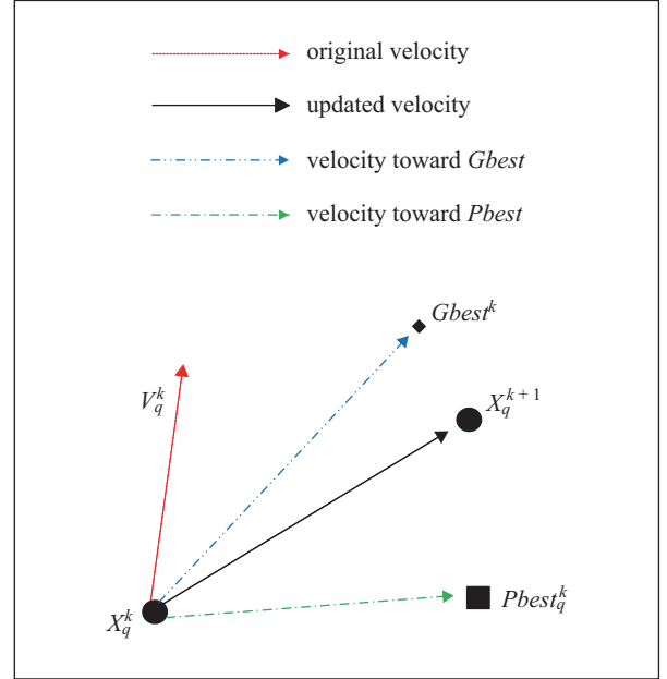
Fig. 3. Depiction of the velocity and position updates in the traditional PSO.
