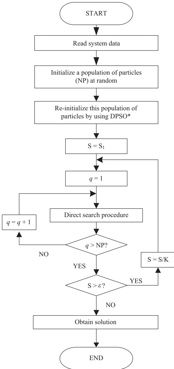
Fig. 6. Simplified flow chart for the proposed hybrid DPSO*-EDSM algorithm.
