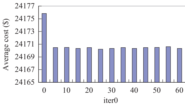
Fig. 7. Comparison of average costs under various iter0 for the system Example 1.
