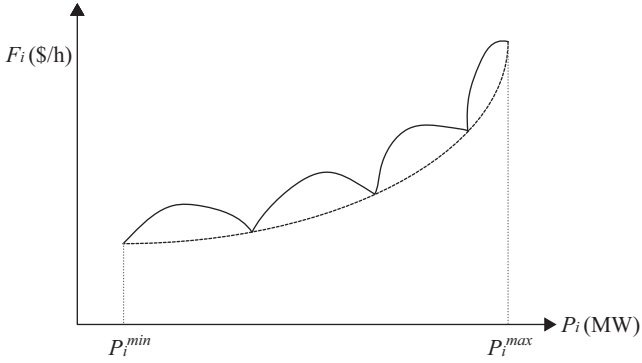
Fig. 2. Fuel cost curve of units with valve-point effects.
