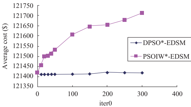
Fig. 9. Comparison of average costs under various iter0 of the two PSO strategies for the system Example 2.
