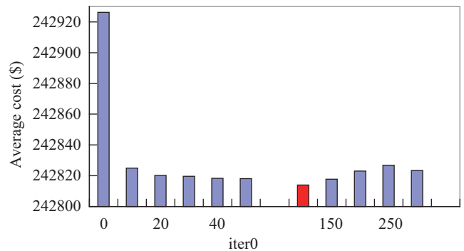
Fig. 11. Comparison of average costs under various iter0 for the system Example 3.
