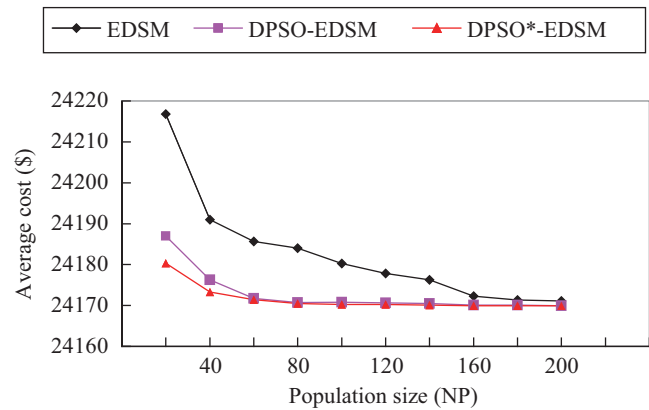
Fig. 8. Comparison of average costs under various NP for the system Example 1.
