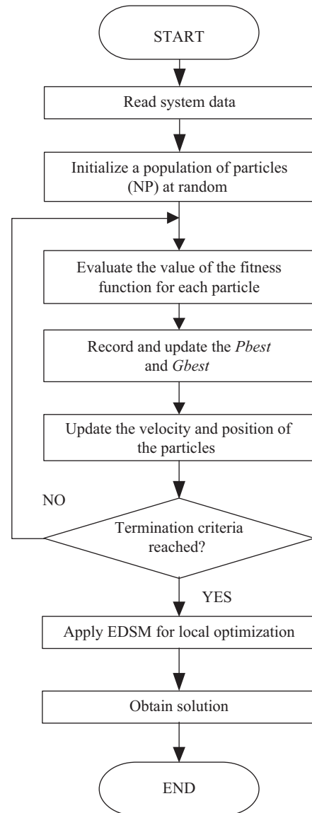
Fig. 5. Simplified flow chart for the conventional hybrid DPSO-EDSM algorithm.
